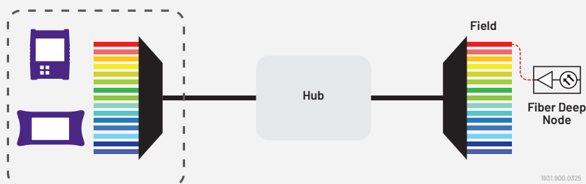
End to end DWDM link characterization: DWDM OTDR
