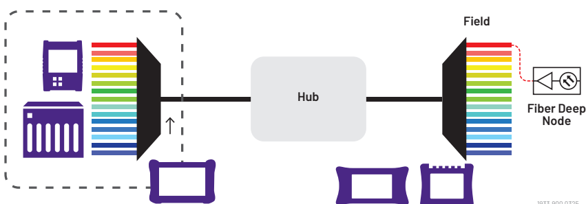
DWDM monitoring and troubleshooting: FTH-9000, DWDM OTDR, DWDM Optical Channel Checker, Nano OSA
