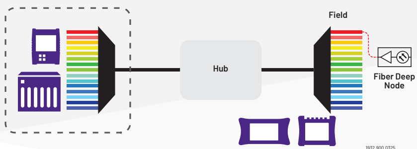
DWDM link wavelength provisioning diagram for DAA Fiber Deep architecture: DWDM Optical Channel Checker, Nano OSA
