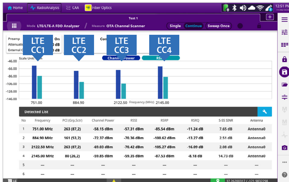
OneAdvisor LTE Signal Analysis – Carrier Aggregation
