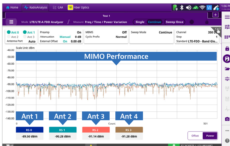
OneAdvisor LTE Signal Analysis – MIMO Power
