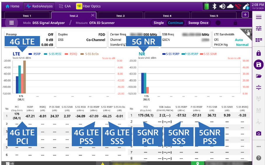
OneAdvisor DSS Signal Analysis – OTA ID Scanner
