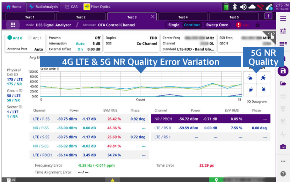
OneAdvisor DSS Signal Analysis – Control Channel
