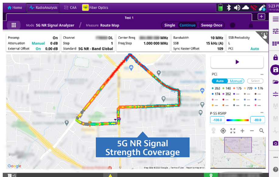
OneAdvisor 5G Signal Analysis – Route Map
