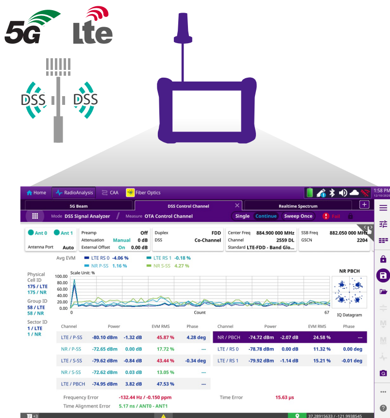
OneAdvisor 800 Dynamic Spectrum Sharing (DSS) Signal Analysis
