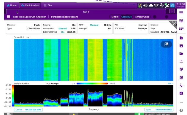
OneAdvisor 800 Real-Time Spectrogram
