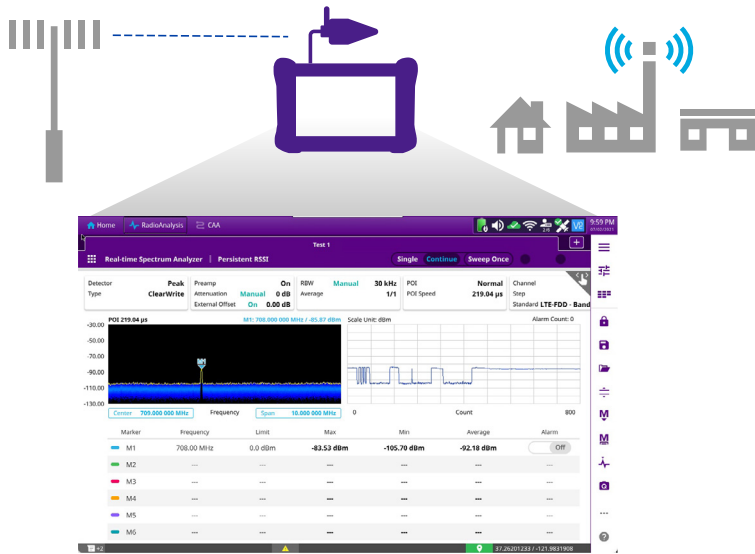
OneAdvisor 800 Interference Analysis (RSSI)
