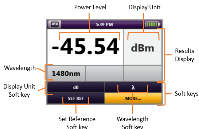
Figure 3: Power Meter Results screen
