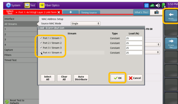
Figure 7: Configure Streams
