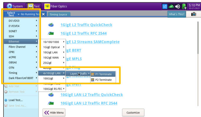
Figure 4: Launch Test
