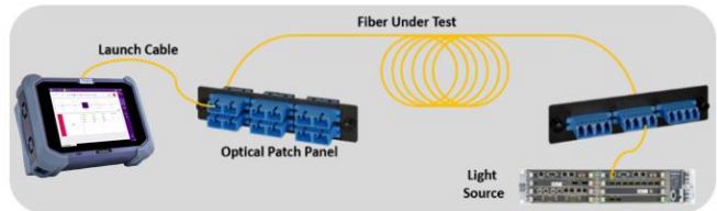
Figure 4: Connecting Reference Cable to OPP
