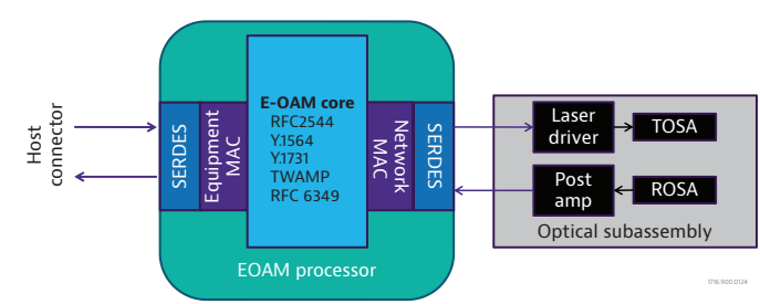
Figure 1. Simplified optical block diagram of JMEP3
