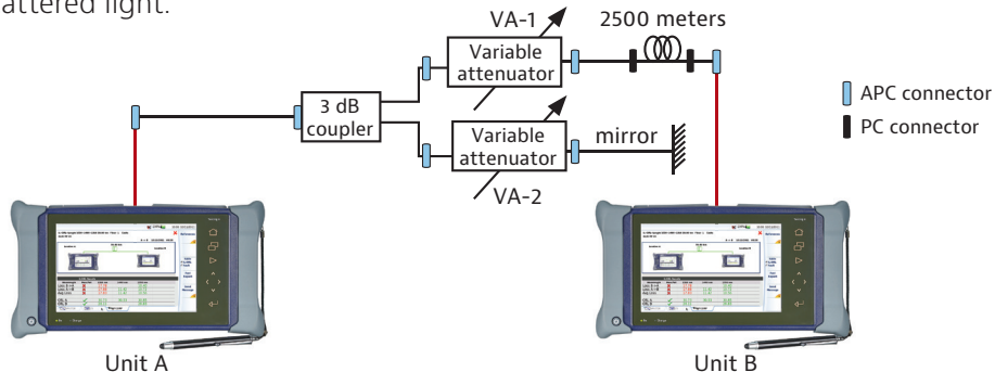
Figure 3. Calibrated link for experimental validation
