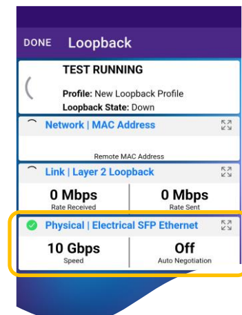
Figure 12: 10G Copper SFP
