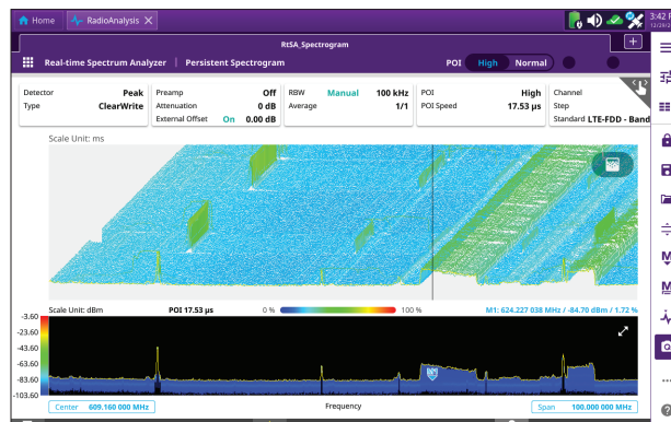
Swept Spectrum interference analysis with 3D Spectrogram
