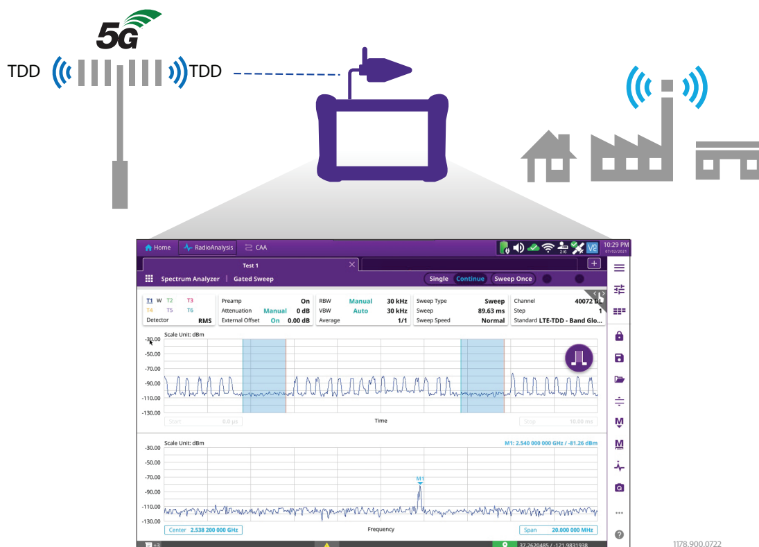
OneAdvisor 800 Dual Gate Spectrum Analysis (TDD Interference)
