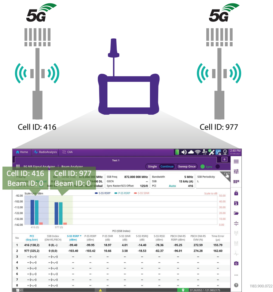
OneAdvisor 800 5G Signal Analysis – Beamforming
