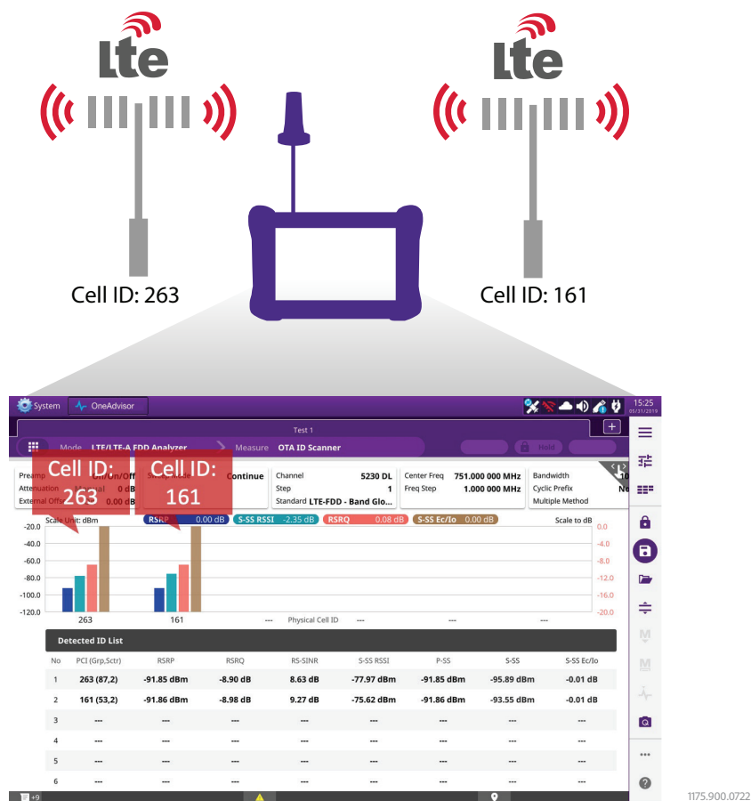
OneAdvisor 800 LTE Signal Analysis
