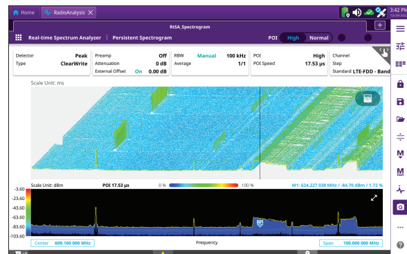
Real-time 3D spectrogram capturing bursty communications
