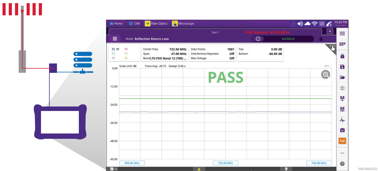
OneAdvisor 800 Coaxial Cable and Antenna Analysis – Return Loss
