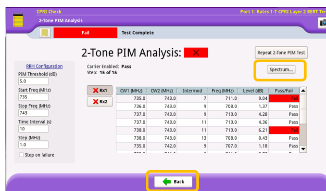
Figure 14: 2-Tone PIM Analysis
