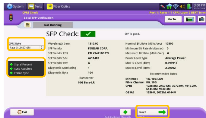
Figure 7: Local SFP Verification
