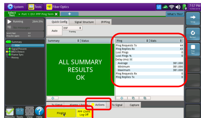
Figure 7: Actions Panel
