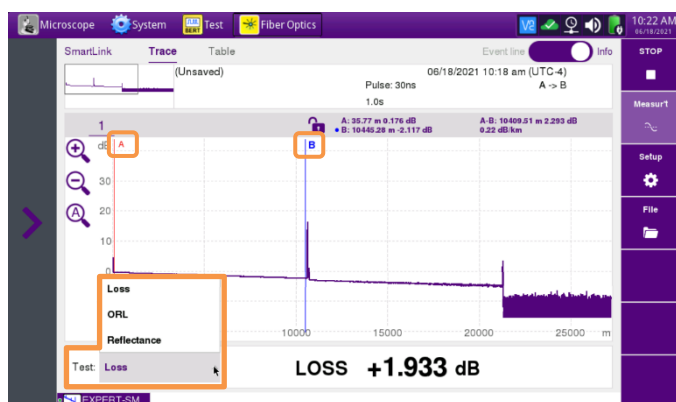
Figure 10: Trace View, Loss Result
