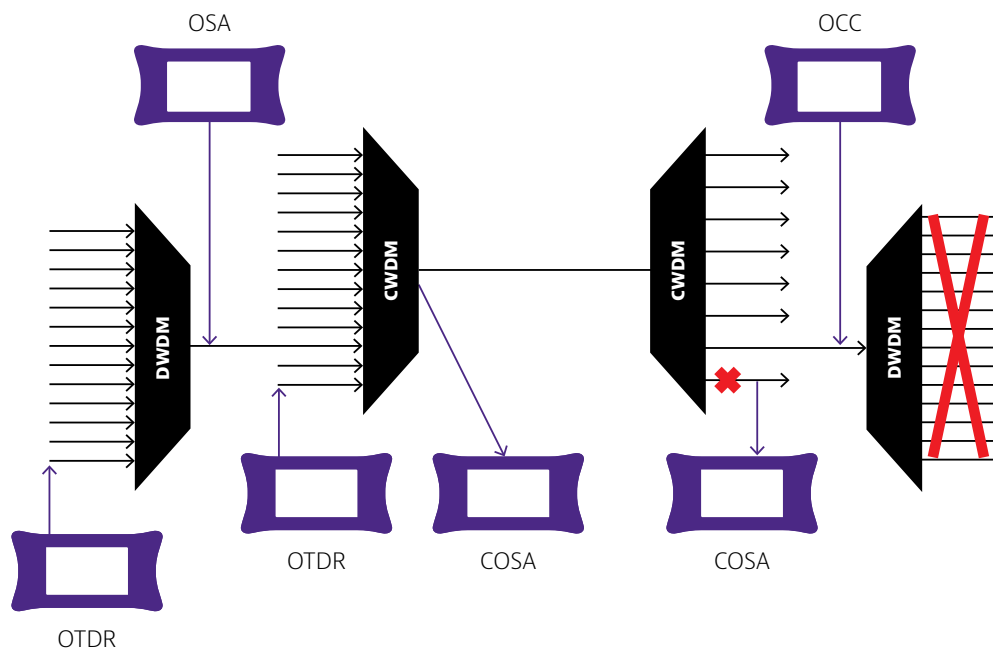
xWDM testing
