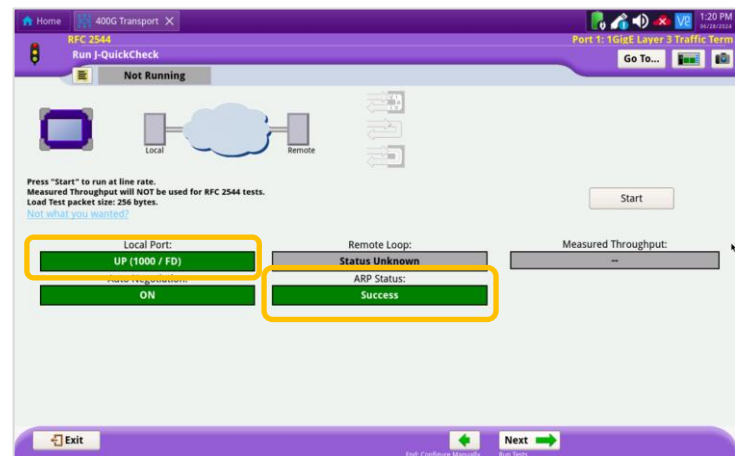
Figure 12: Local Port status
