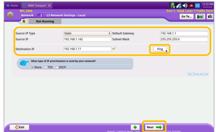
Figure 7: L3 Network Settings - Local
