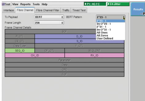
Figure 5. BER test setup
