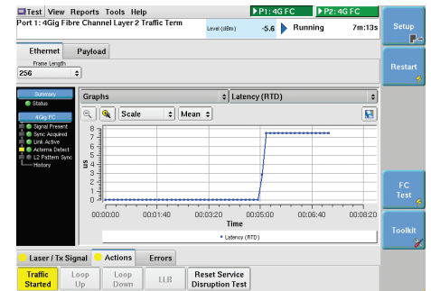
Figure 4. RTD verification
