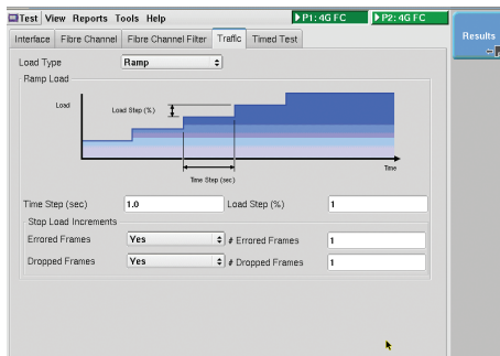
Figure 2. Throughput setup
