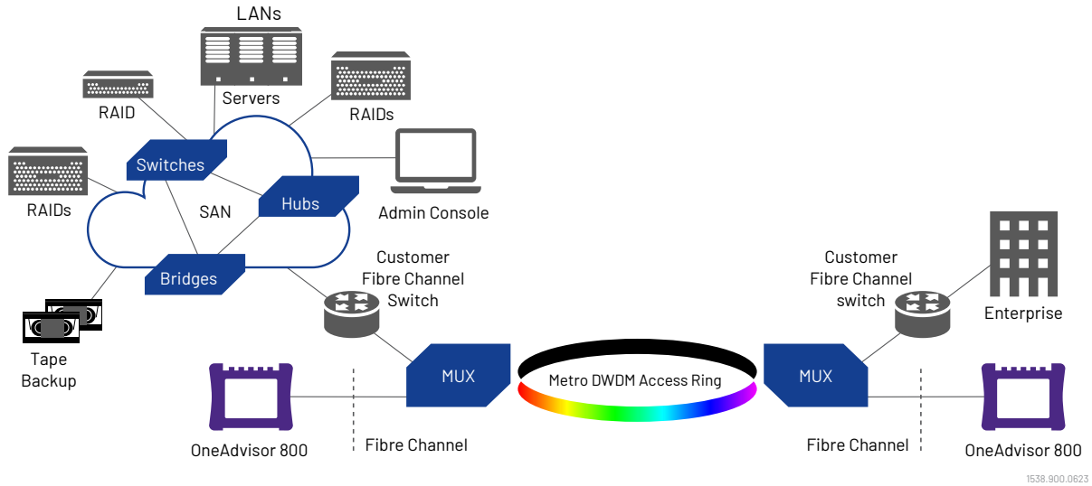
Figure 1. Storage area network
